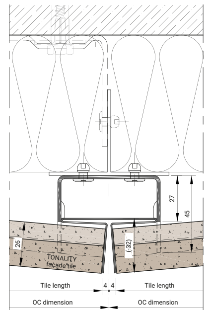
Open joint profile (30 mm) Due to production tolerances, it is possible that the open profile will not end precisely at the tile surface.
