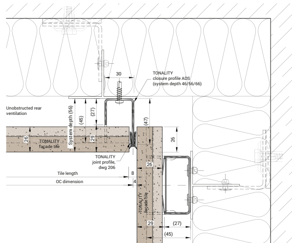
optional: Internal corner 90° with ADS closure and joint profile
